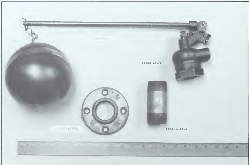
Photo 2. Brass float valve, arm and ball, with fillings. Two steel floor flanges are needed per assembly. All components are 1 1/2-inch diameter.
